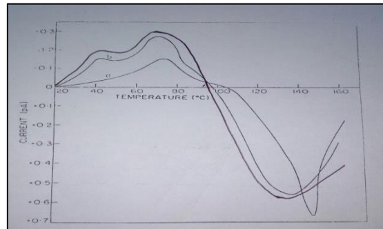
Fig 4: Three Typical Short Circuit TSC Curves Charged to Initial Surface Potentials of -300V (curve a), -800V (curve b) & 1200 (curve c)
