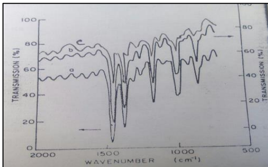
Fig 4B: Infrared of Virgin (Spectra a), Hexane Treated (Spectra b) BOPP & TOPP
