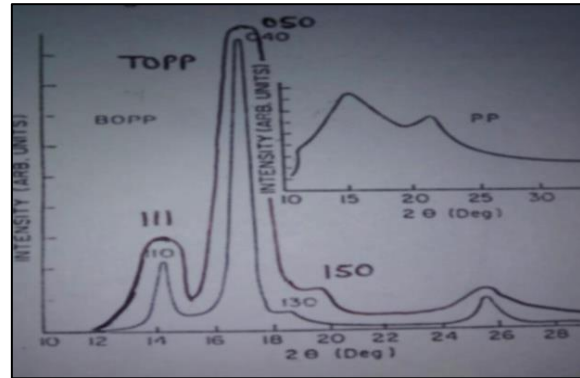
Fig 1:- X-ray Scan for BOPP & TOPP
