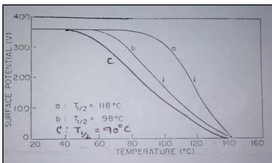
Fig 3: TSDP of TOPP, BOPP & PP. Samples Negatively
